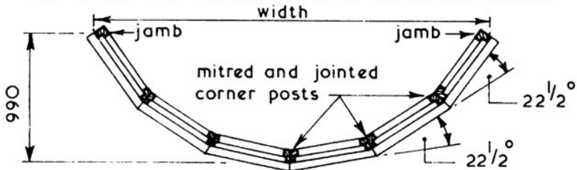
TYPICAL 6 LIGHT CIRCULAR OR SEGMENTAL BAY WINDOW
