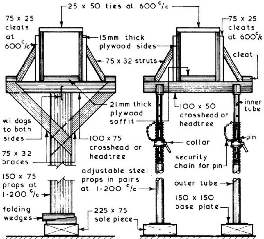
SINGLE PROP SUPPORT
