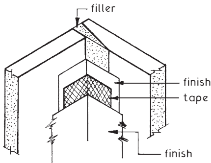
Internal Corner
