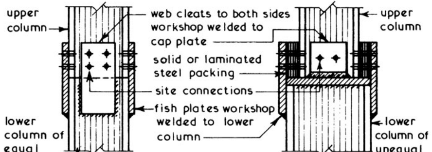
COLUMN TO COLUMN CONNECTIONS
