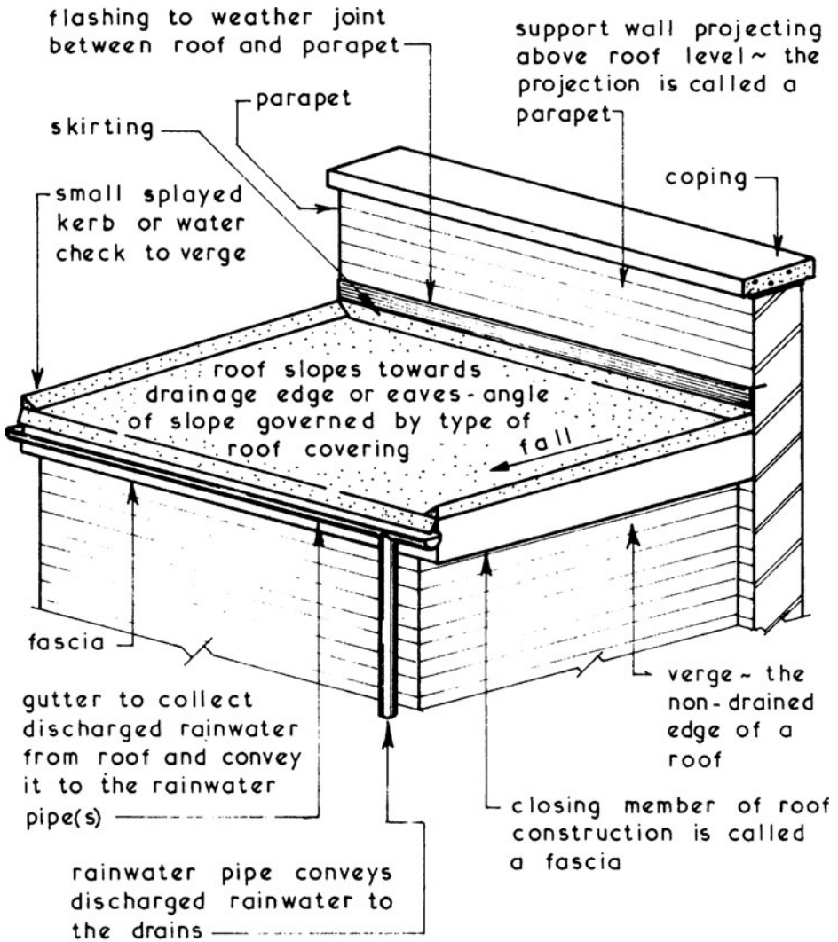
FLAT ROOFS
