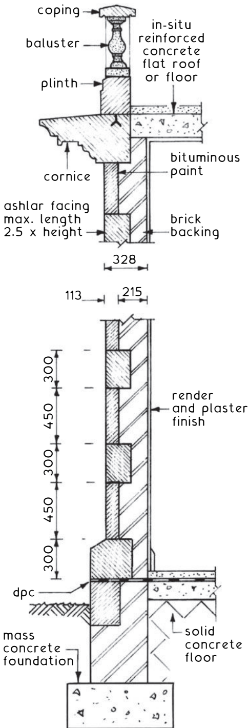
Example of existing ashlar stonework (dimensions in mm)
