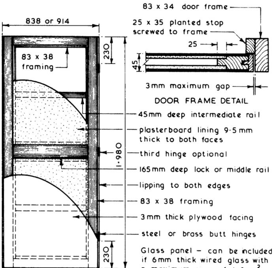
SECTIONAL ELEVATION
