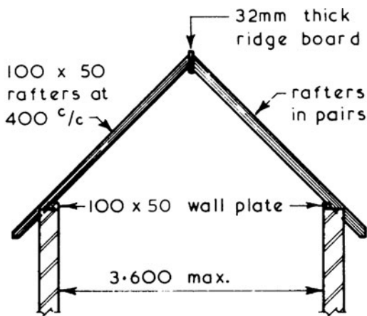
COUPLE ROOF
