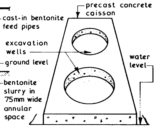
MONOLITHIC CAISSON
