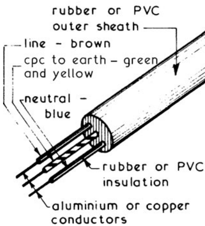
SHEATHED CABLES
