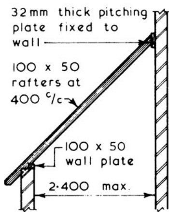
LEAN-TO ROOF
