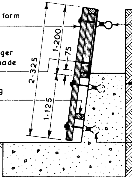
STAGE TWO OR SECOND LIFT
