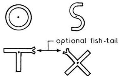
Common decorative iron pattress plates and straps
