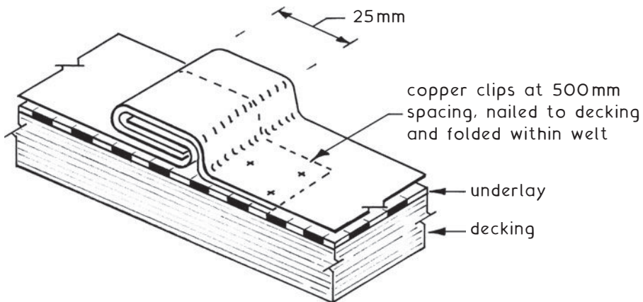
Welted joint
