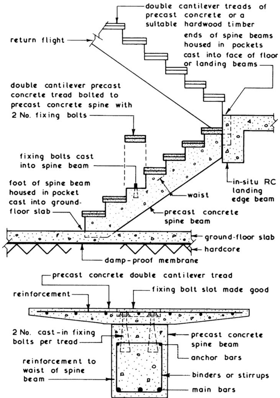
TYPICAL SECTION
