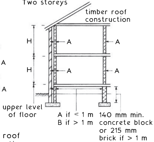
Two storeys
