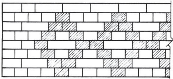
DUTCH BOND
