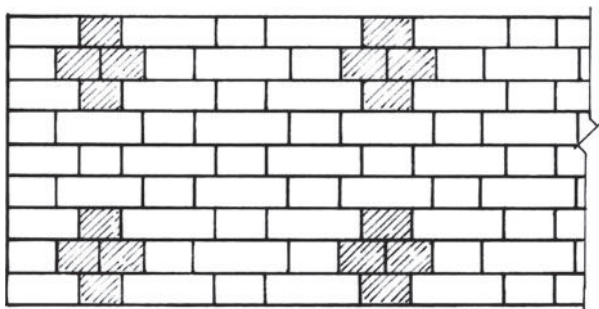
FLEMISH CROSS BOND
