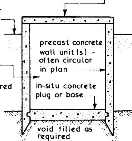
OPEN CAISSON
