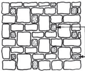
Squared random rubble with through snecks
