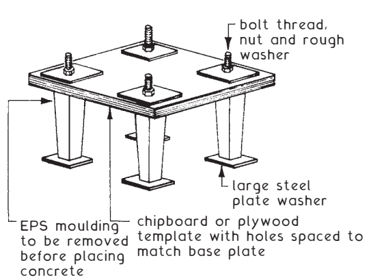
BOLT BOX
