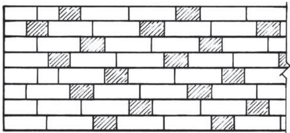
MONK BOND
