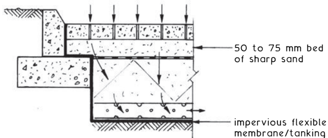
Subgrades of no capacity for infiltration
