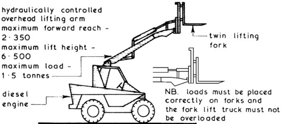
OVERHEAD FORK LIFT
