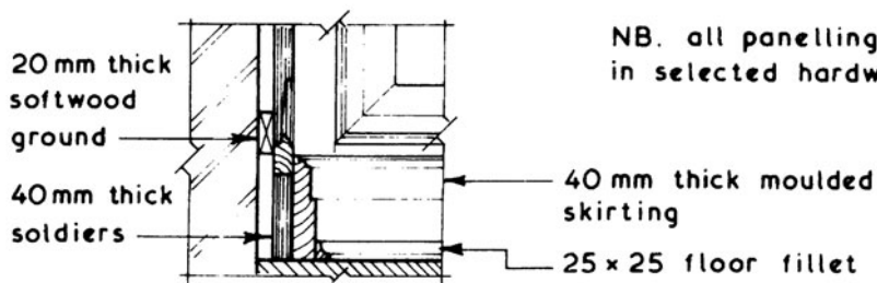
SECTION
