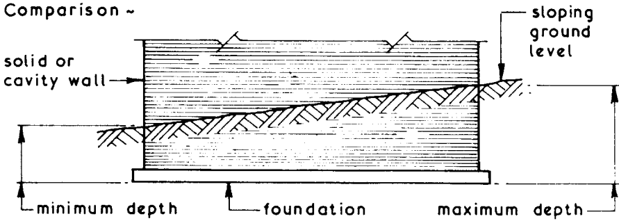
LEVEL FOUNDATION
