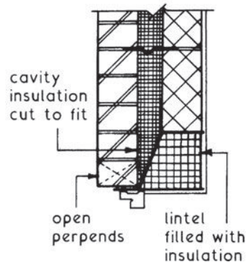
WINDOW/DOOR HEAD
