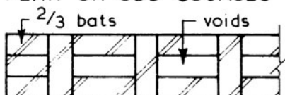
RAT TRAP BOND - uses brick on edge courses - hollow pockets or voids reduce total weight of wall and by the bricks on edge there is an overall saving of materials.
